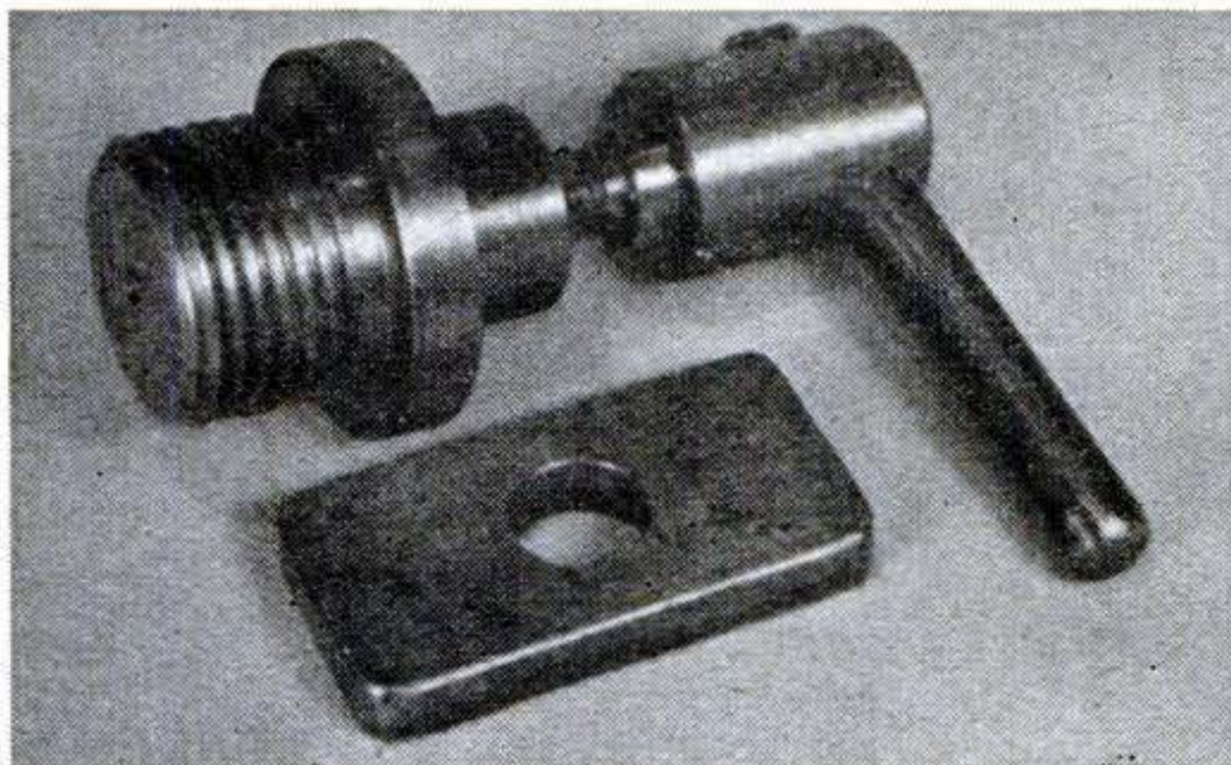
These three parts are all you need to mount lathe chucks or faceplates on the drill press.
